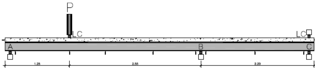
Figure 3. The load at the maximum positive moment of sections for the restrained steel-concrete composite beams.
