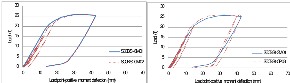
Figure 4. The relationship between loading capacity and deflection capacity (a) SCCB-S-SM-01 and SCCB-S1-CM-02; (b) SCCB-S-SM-01 and SCCB-S1-CP-03.
