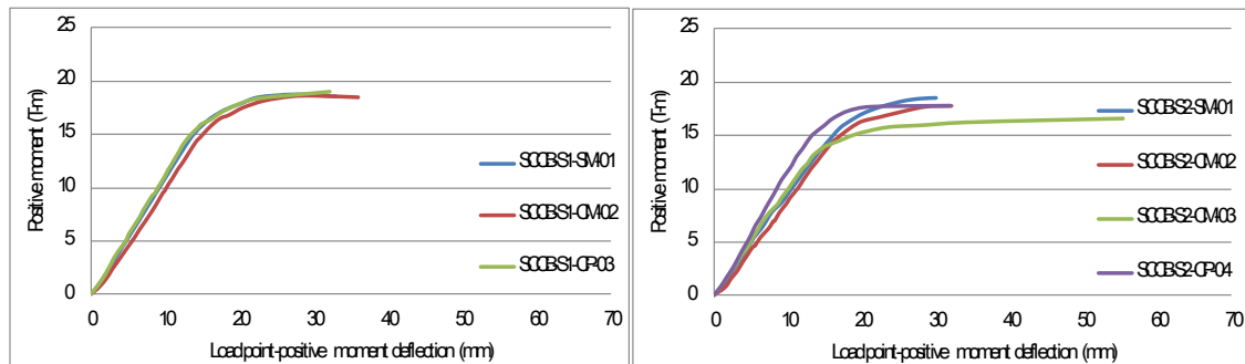
Figure 7. The envelop curves of restrained steel-concrete composite beams (a) Fully composite beam (b) Partially composite beam.
