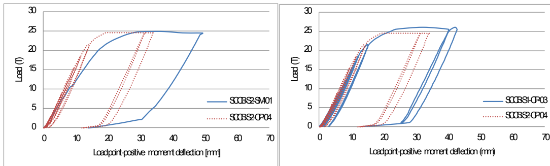
Figure 6. The relationship between loading capacity and deflection capacity (a) SCCB-S1-SM-01 and SCCB-S2-CP-04 (b) SCCB-S1-CP-03 and SCCB-S2-CP-04.
