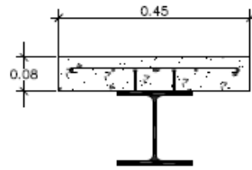
Figure 1. The restrained steel-concrete composite beams.
