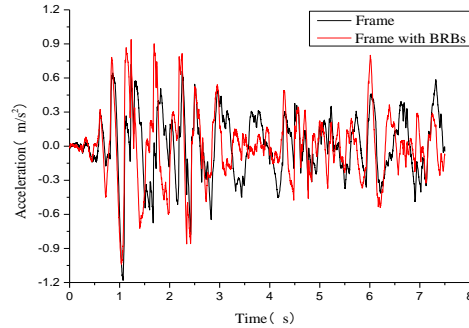
Figure 7. Acceleration-time curves of top story under 70 gal (EL_CENTRO).
