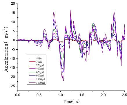
Figure 6. Acceleration-time curves of top story in SY-2 under ranged PGA.
