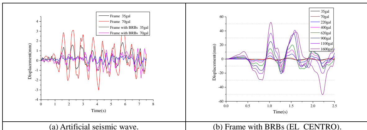
Figure 5. Displacement-time curves of 3 rd story.
