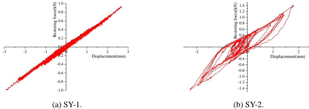
Figure 8. Hysteresis loops of 3 rd story under 70 gal.
