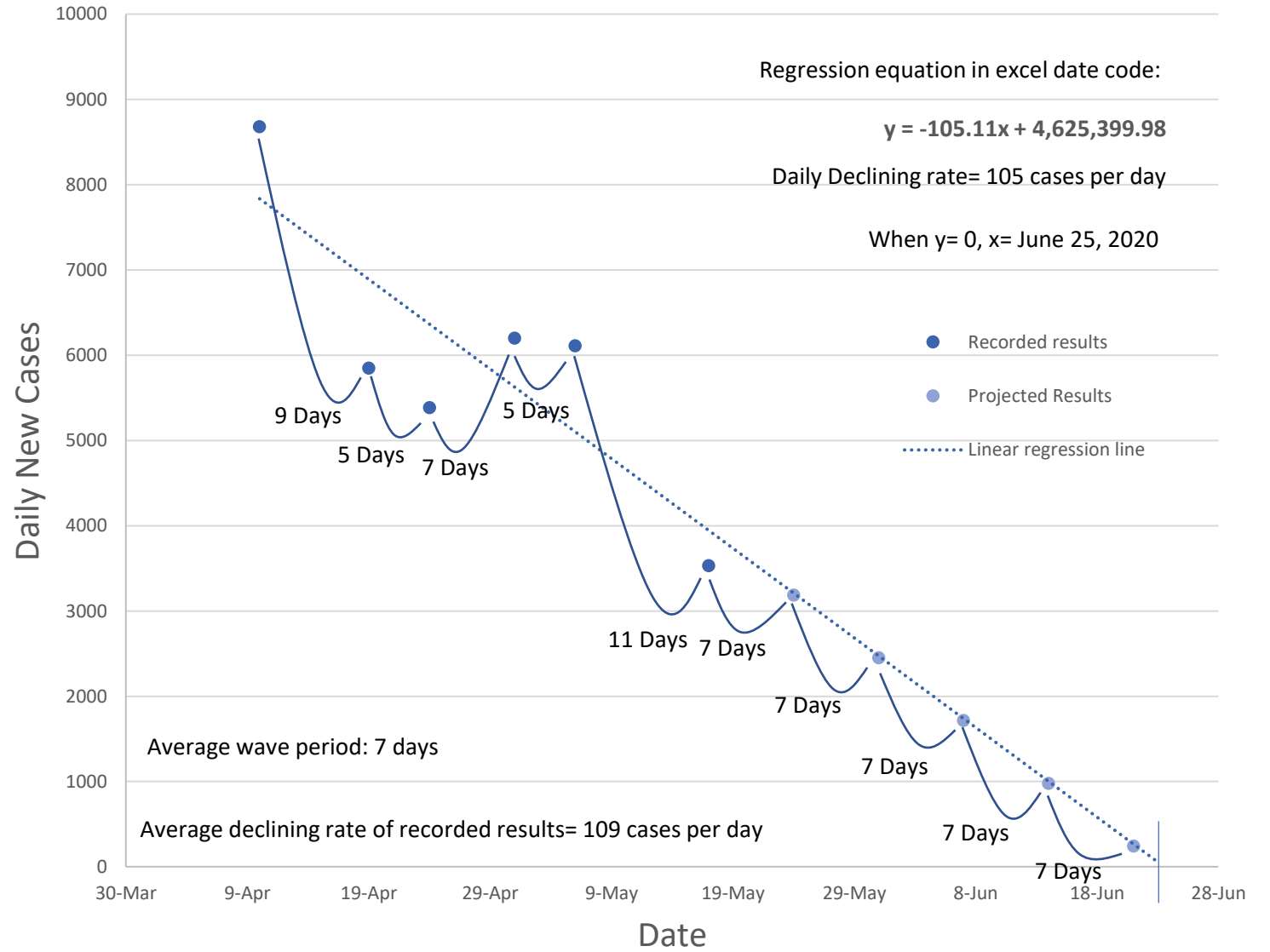
Regression Line of Peak Periods: Cyprus
