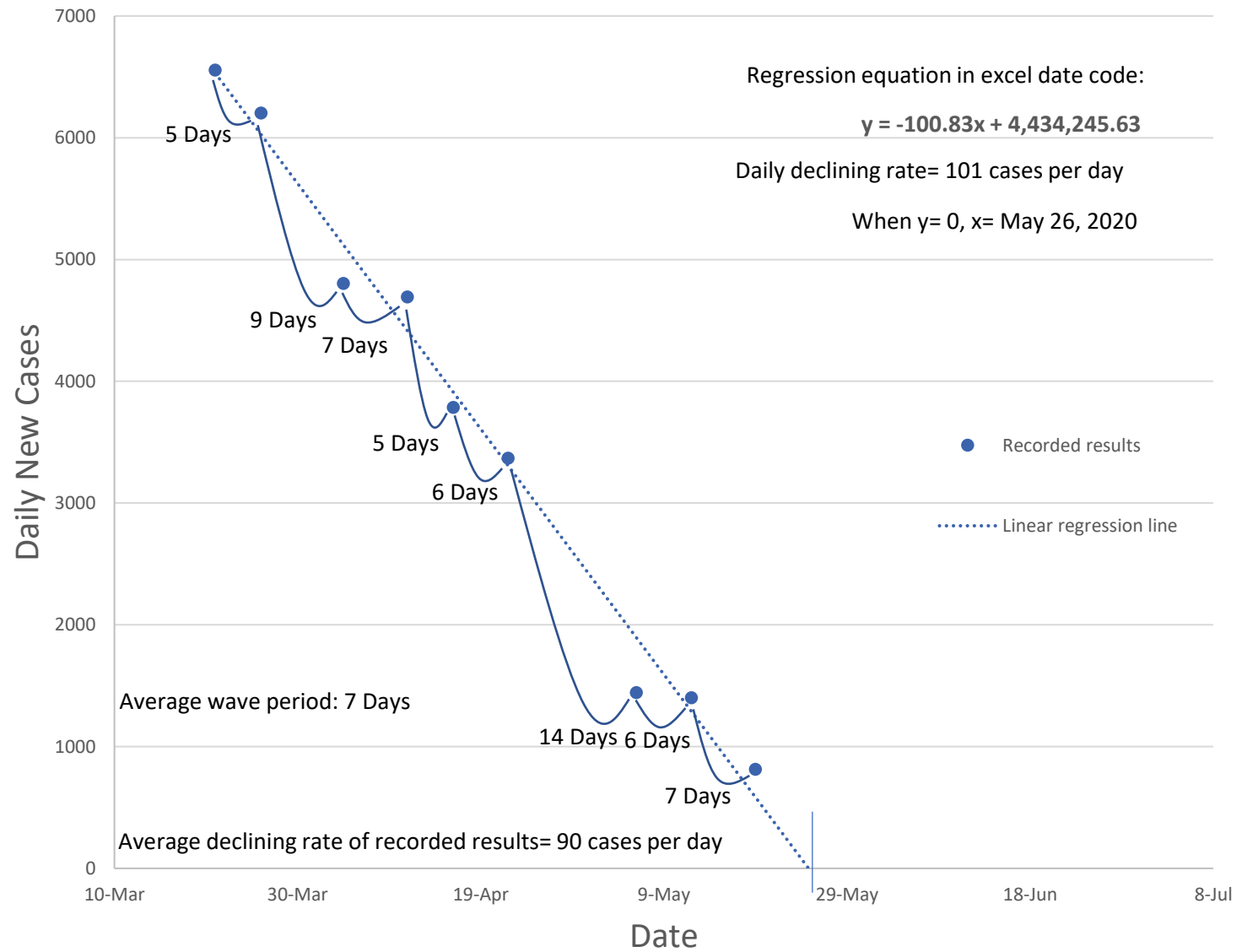
Linear Regression of Peak Periods: Italy
